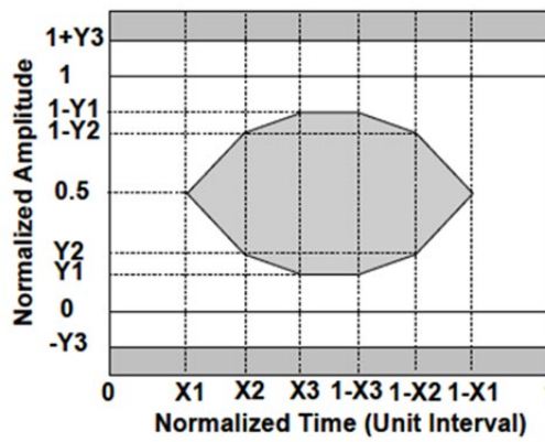
Figure 4. Eye Mask Definition
