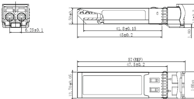
APSPCxxB33CDL40
