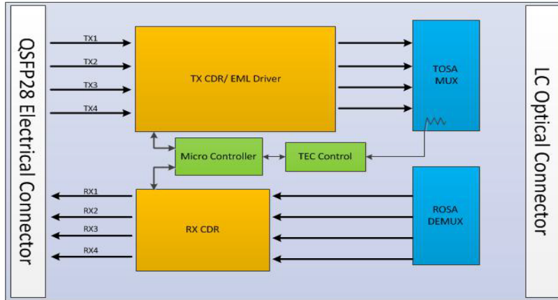
Figure 1. Transceiver Block Diagram
