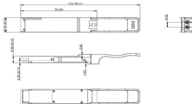
Figure 4. Mechanical Outline
